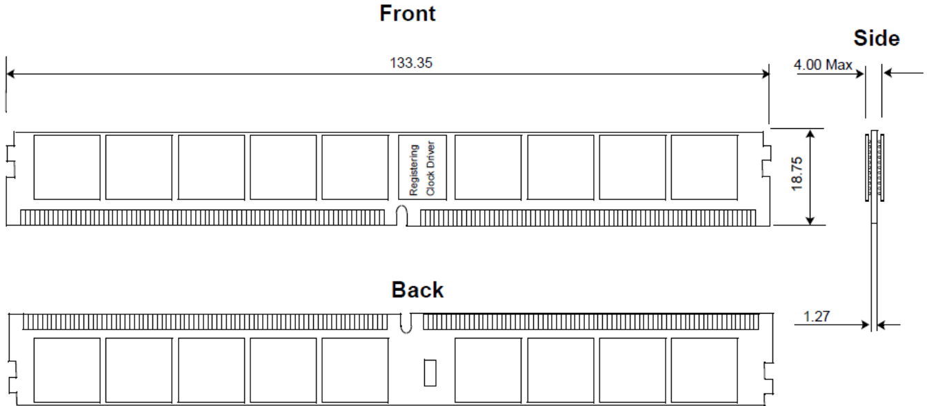
Figure 1 - Package Dimensions
