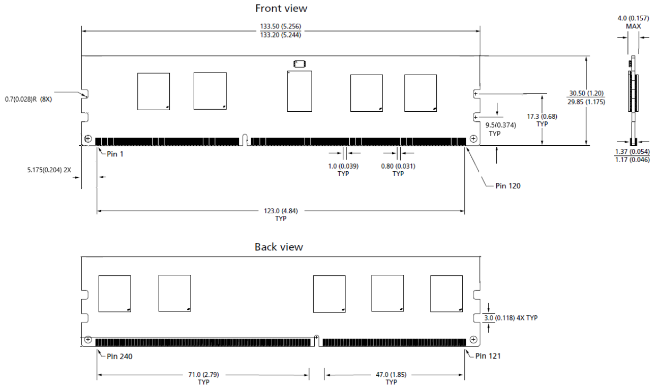
Figure 1 - Package Dimensions
