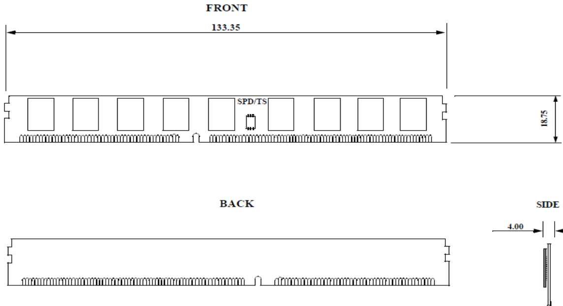
Figure 1 - Package Dimensions
