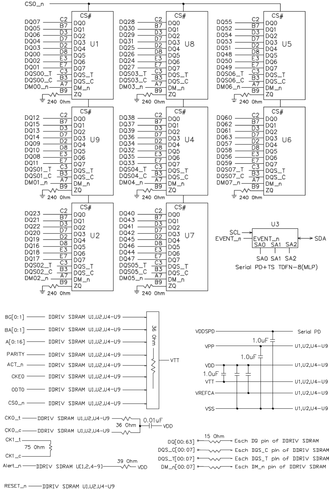
Figure 1 - Function Block Diagram_SCE16GS03H2F1C-32AA
