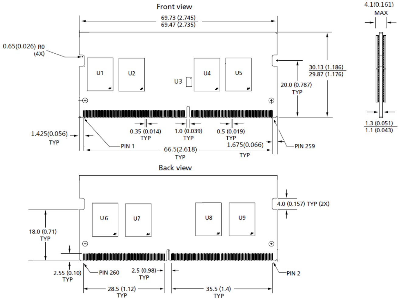
Figure 2 - Package Dimensions_SCE16GS03H2F1C-32AA
