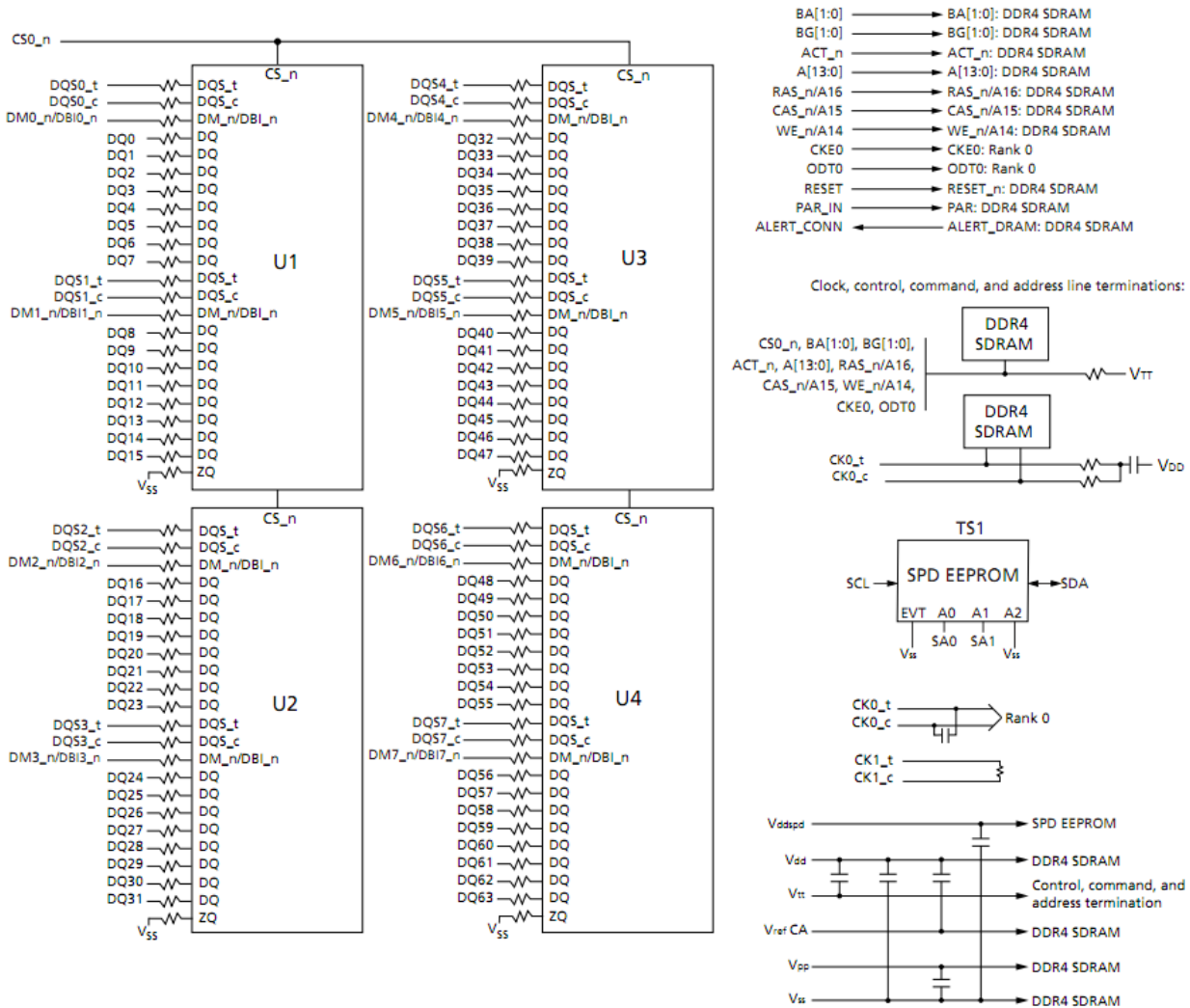
Figure 1 - Function Block Diagram_SCE08GS04M1F1C-32AA
