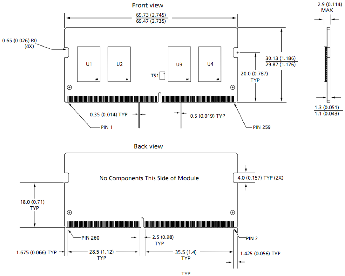
Figure 2 - Package Dimensions_SCE08GS04M1F1C-32AA
