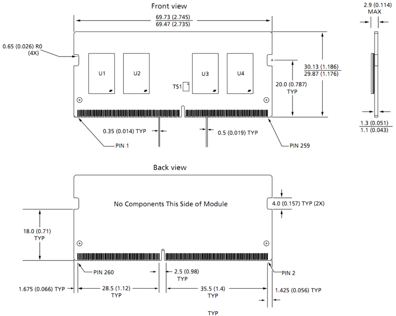
Figure 2 - Package Dimensions_SCQ08GS04M1F1C-32AA
