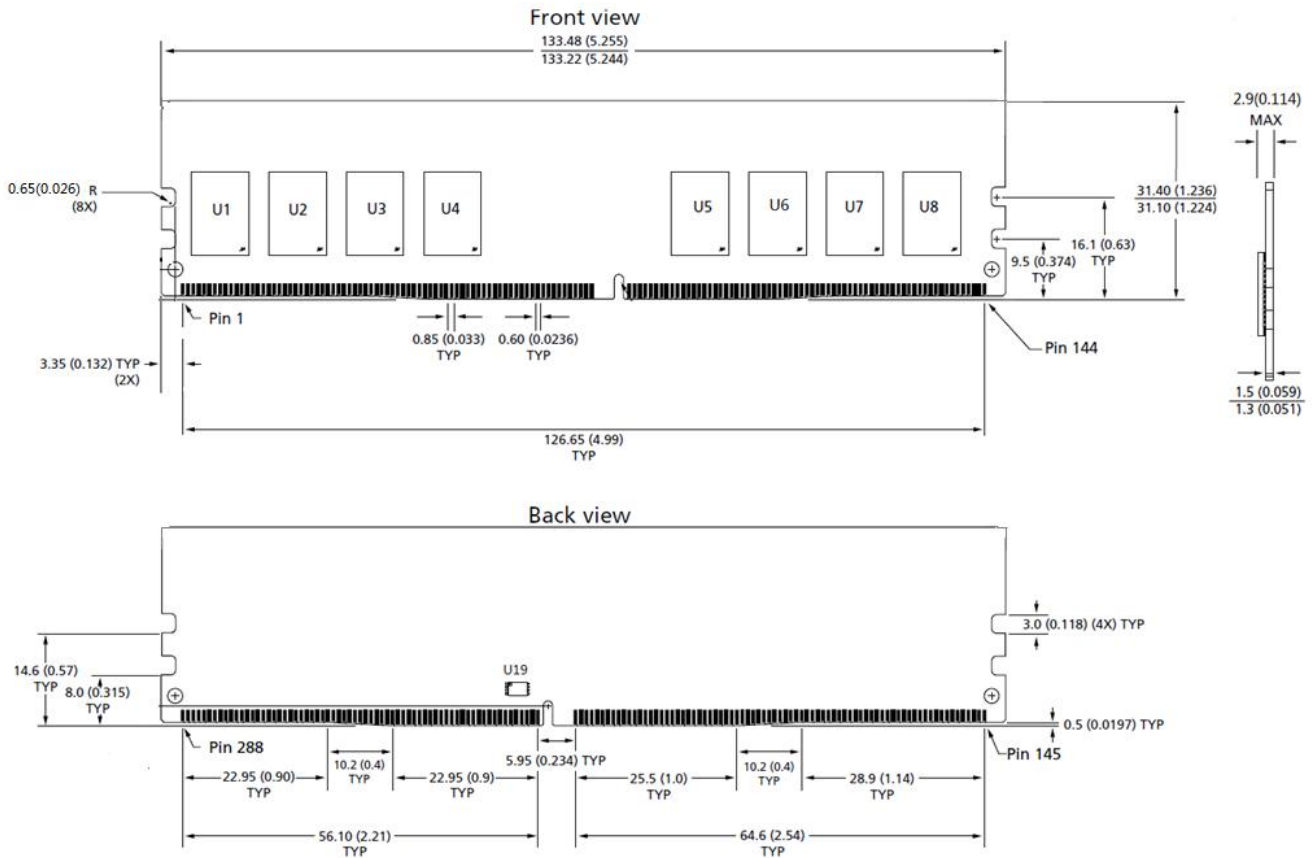
Figure 2 – Package Dimensions_SCQ08GU03M2F1C-32AA
