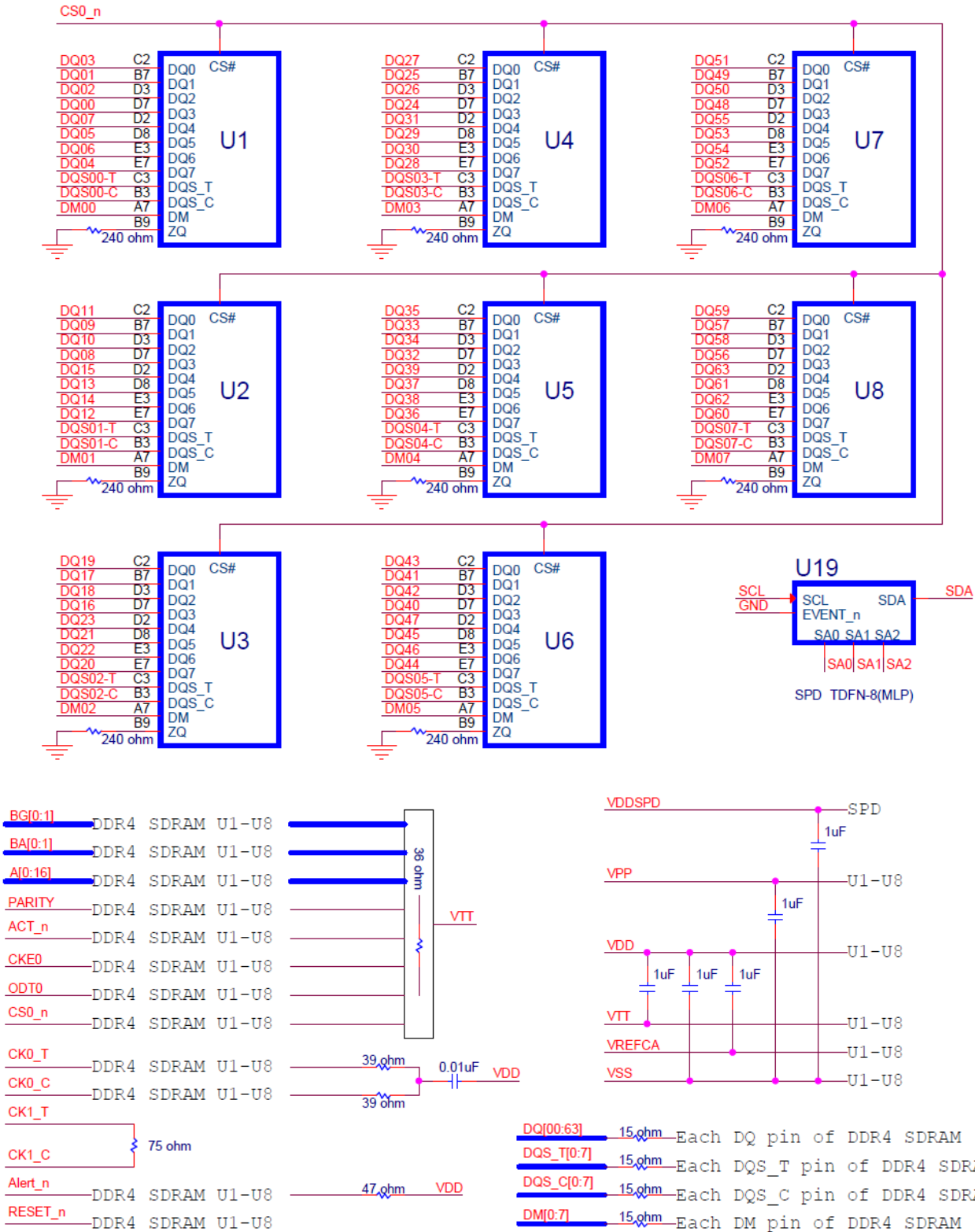
Figure 1 – Function Block Diagram_SCQ08GU03M2F1C-32AA
