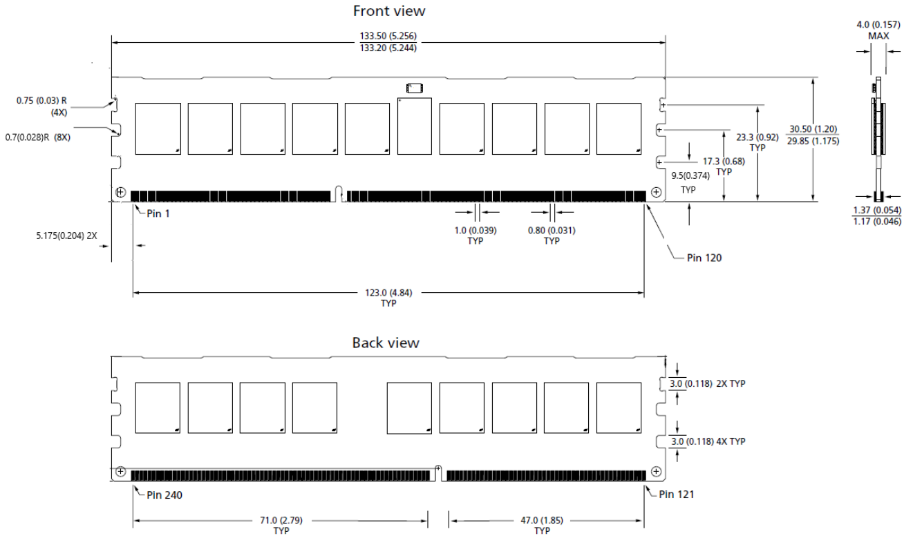
Figure 1 - Package Dimensions_ HXMSH8GP13A2F1CL16K
