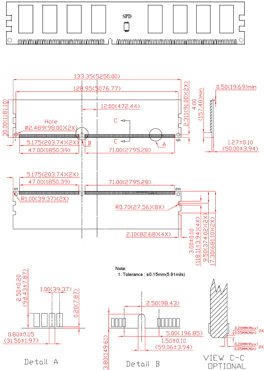
Figure 1 - Package Dimensions
